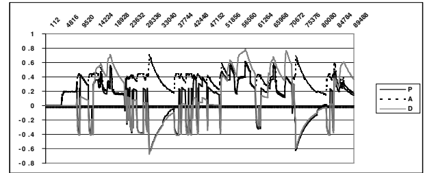
Figure 6: PacMan using both banks, 100ms instrumentation
